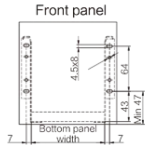
Front panel / Back panel
