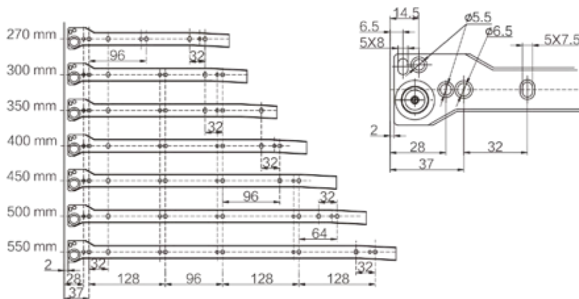
Fastening position for cabinet member / Drilling pattern for cabinet member
