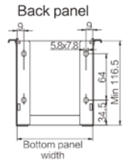
Installation measurement
