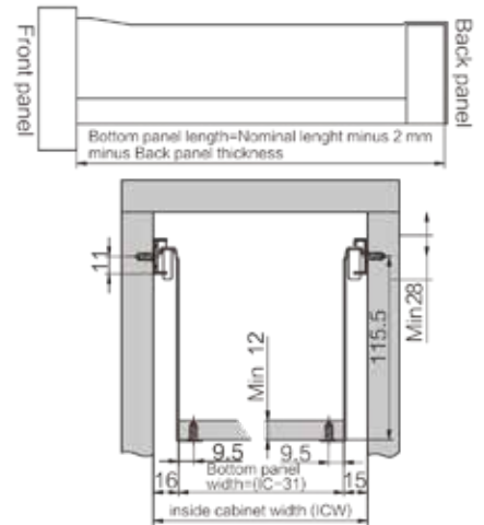
Installation measurement
