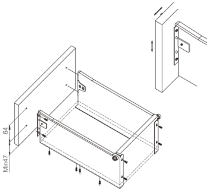
Assembling Diagram / Front adjustment Diagram
